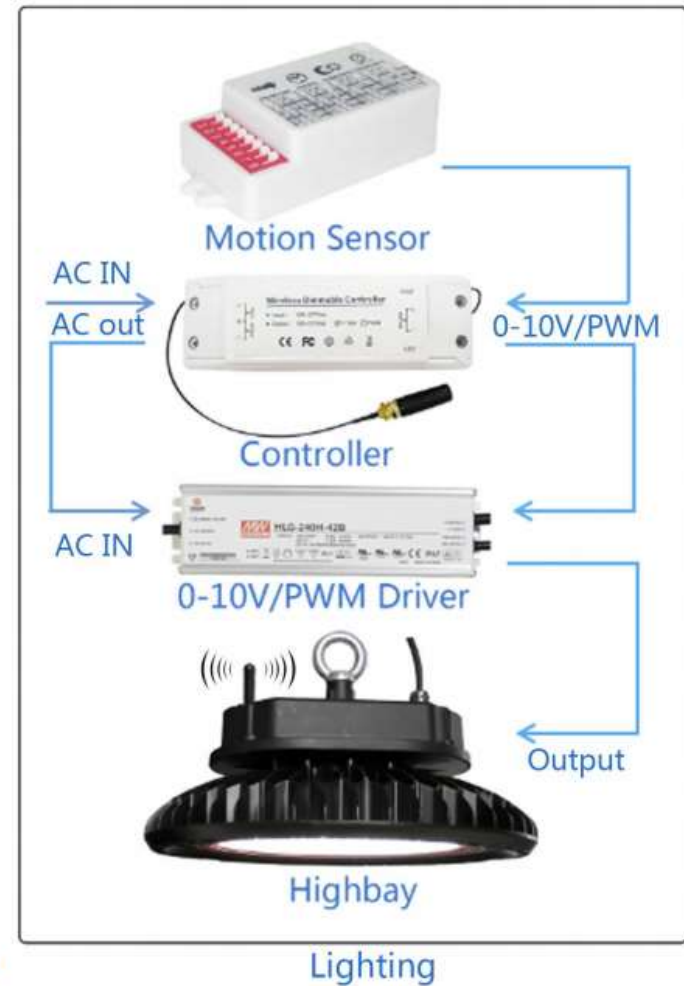
System Diagram
